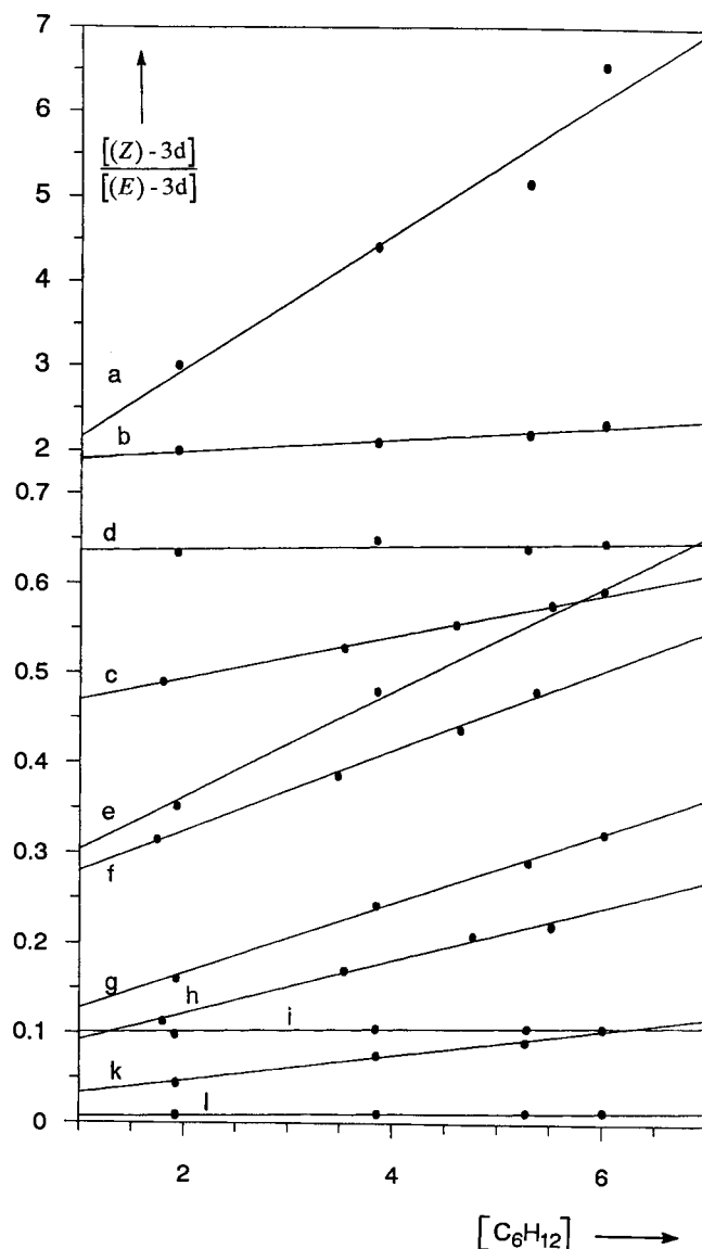
Figure 2. Dependence of the ratio of the addition products [( Z )- 3 ]:[( E )- 3 ] on the concentration of the hydrogen donor cyclohexane at 240 °C (The ratio of the addition products to the alkynes 1d , 1f , and 1h was measured at 260 °C.)
