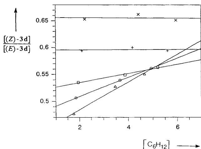
Figure 5. Dependence of the ratio of the addition products [(Z)- 3d ]:[(E)- 3d ] on the concentration of the hydrogen donor cyclohexane from 200 to 260°C. x: 200°C, +: 220°C, □: 240°C, ○: 250°C, Δ: 260°C
