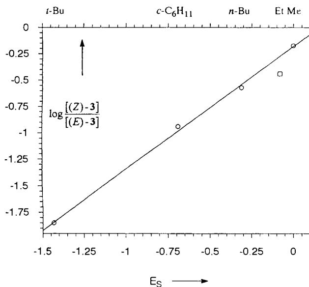
Figure 4. Correlation of the stereoselectivity of the addition of cyclohexane to 1-alkynes 1e, 1g, 1k, 1l (240°C), and 1h (260°C) with steric substituent constants E_S of the alkyl substituents
